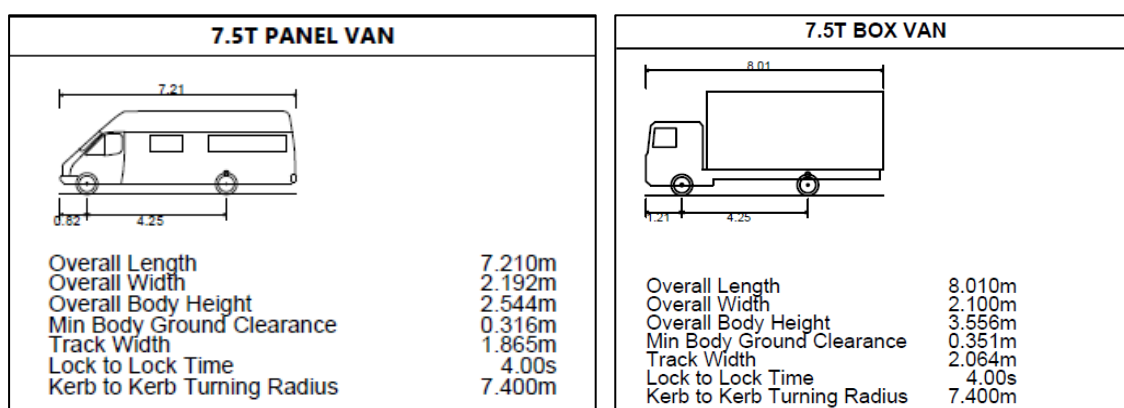
Figure 3.3: Examples of Infrequent Larger Servicing Vehicles
