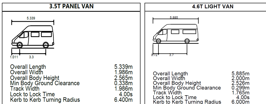
Figure 3.2: Examples of Typical Daily Servicing Vehicles
